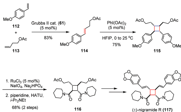
Scheme 17 Oxidative radical dimerization in the total synthesis of (±)-nigramide R.
