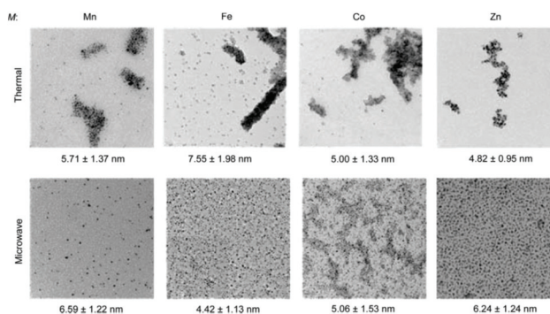
Fig. 18 TEM images of MFe 2 O 4 nanoparticles synthesized by the thermal and microwave synthetic routes. For all the investigated cases, the microwave synthesis produces highly homogeneously dispersed nanoparticles. The numbers below each image display the average nanoparticle size with its deviation. Reproduced with permission from Solano et al. 331
