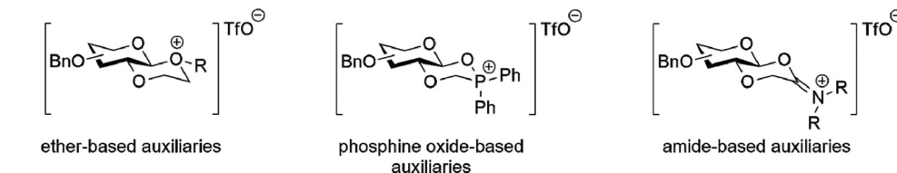
Fig. 1 (A) The two main strategies for stereoselective glycosylation. The oxocarbenium ion is trapped either by a C-2 auxiliary or additive to control the structure of the reactive intermediate. (B) Newly developed C-2 auxiliaries based on common additive functional groups.
