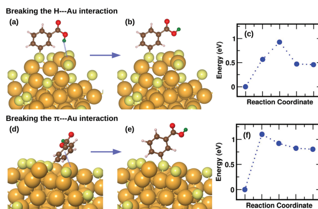
Fig. 5 (a) The optimized structure of Au 68 ( m -MBA) 32 highlighting a COOH...Au interaction. (b) The ligand in (a) is modified such that the carboxylic H is pointed away from the Au core breaking the interaction. (d) The optimized structure of Au 68 ( m -MBA) 32 highlighting a \pi ...Au interaction, (e) the structure with the ligand in (d) modified such that it stands upright breaking the interaction. (c) and (f) show the energy profiles as obtained from CI-NEB calculations for the minimum energy pathway from structure (a) to (b), and (d) to (e), respectively. Au, S, C, O, phenyl H and carboxylic H are shown in golden, pale yellow, brown, red, white and green colors, respectively. All the ligands were included in the calculation but the other ligands are not shown for clarity.
