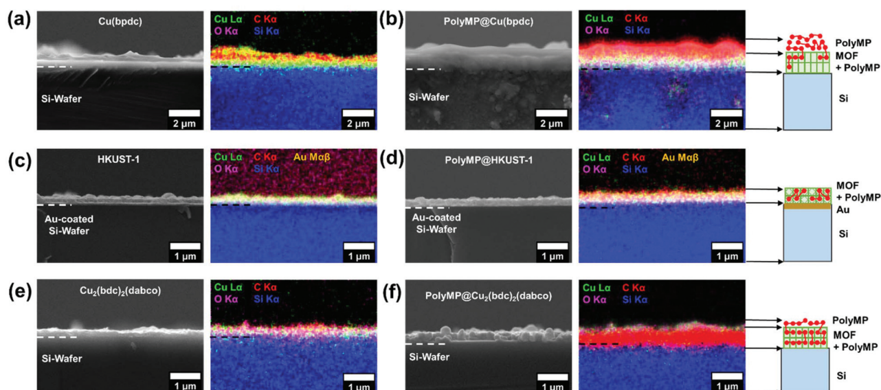
Fig. 3 SEM images and the corresponding EDXM of (a) pristine 1 , (b) polyMP@1 , (c) pristine 3 , (d) polyMP@3 , (e) pristine 2 , and (f) polyMP@2 . For 1 and polyMP@1 , the formation of a clear, strong top-layer is visible, whereas for 3 and polyMP@3 , no top-layer formation is observed. Note that due to the strong intensity of carbon from (e) to (f), the MOF signal almost diminishes, but from the thickness difference, we assume the formation of a small top-layer. The cartoons on the right side of (b), (d) and (f) show the observations of polyMP formation.
