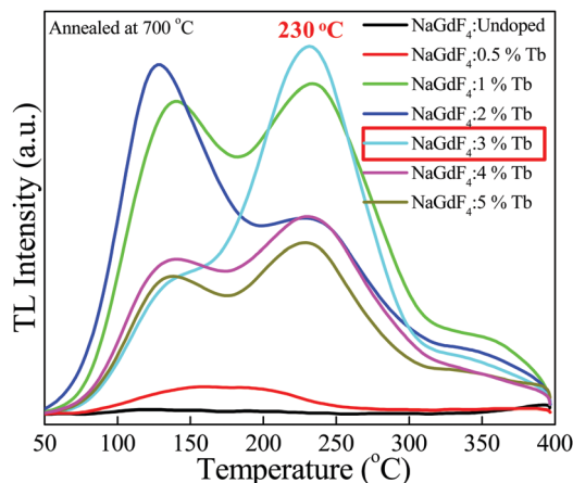
Fig. 8 Thermoluminescence glow curve optimization of the NaGdF 4 :x% Tb 3+ ( x = 0, 0.5, 1, 2, 3, 4, 5 ) phosphor annealed at 700 °C, irradiated at a gamma dose of 1 kGy. NaGdF 4 :3% Tb 3+ showed the most suitable glow curve at 230 °C.
