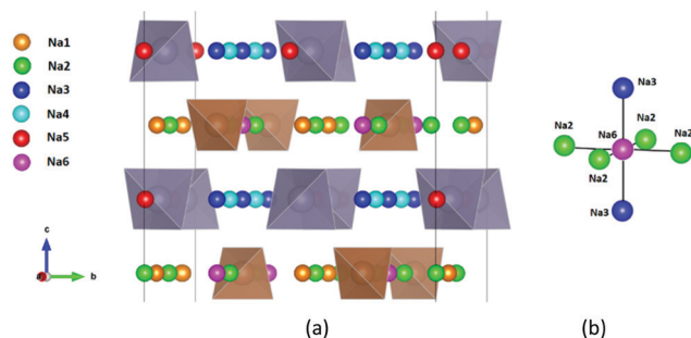
Fig. 1 Distribution of Na sites in the structure of \text{Na}_{11}\text{Sn}_2\text{PS}_{12} : (a) overview of Na site distribution in one half of the unit cell projected approximately on the b–c plane. Grey (brown) tetrahedra represent \text{SnS}_4 (PS 4 ), coloured spheres the partially occupied Na sites (Na1 (16f) orange, Na2 (32g) green, Na3 (16d) dark blue, Na4 (16c) light blue, Na5 (16e) red and Na6 (8b)). The naming of the Na sites follows ref. 46. (b) Detail of the structure model highlighting the local Na sites adjacent to the low occupancy site Na6. This cluster of Na sites will be referred to as the (\text{Na}_2)_4(\text{Na}_3)_2\text{Na}_6 site cluster below, while the 3 Na sites Na1, Na4 and Na5 not involved in the cluster will be referred to as “matrix sites”.
