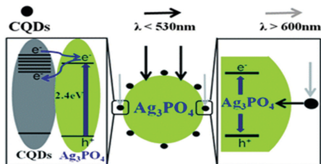
Fig. 5 Schematic representation corresponding to Cdote assisted improved photocatalytic activity of a Cdote/Ag 3 PO 4 complex. Reprinted with permission from ref. 115. Copyright 2012 Royal Society of Chemistry.
