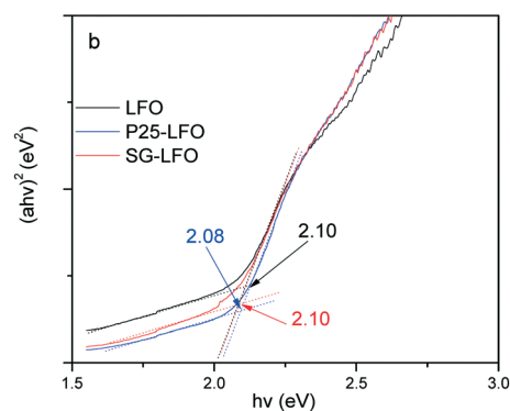
Fig. 3 UV-vis diffuse reflectance spectra (a) and Tauc plots (b) of the LFO, P25-LFO and SG-LFO catalysts. The numerical values in (b) indicate the band gap energies estimated from the Tauc plots.
