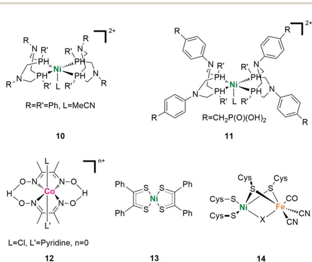
Fig. 10 Representative structures of Ni-based, Co-based HECs and the active centre of [NiFe]-H 2 ase.
