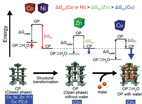
Fig. 3 Proposed energy diagram for the structural transformation. If the \Delta G_{ST} values for CoCID-1 and NiCID-1 are much larger than proposed, OP \supset H 2 O for CoCID-1 and NiCID-1 will be more unstable than OP for ZnCID-1 and CuCID-1, which cannot be confirmed from the experimental results.
