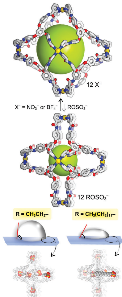
Scheme 1 Encapsulation of ROSO_3^- ( R = \text{ethyl-, octyl-, decyl-, dodecyl-, and tetradecyl-} ) within present spherical coordination cages and different surface tensions depending on included alkyl chains of surfactant.
