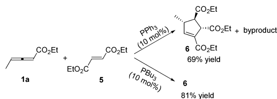
Scheme 2 Phosphine-catalysed (3+2) cycloaddition reactions of acrylate, vinyl phenyl sulfone or fumarate with \gamma -methyl allenate.
