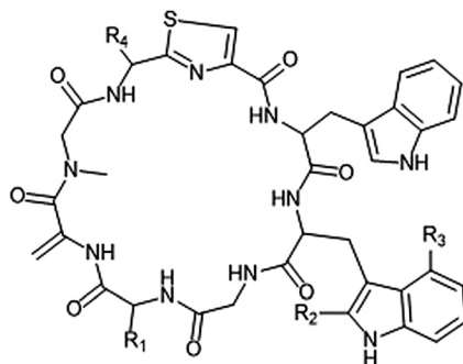
Argyrin A (30): R_1 = \text{CH}_3 , R_2 = \text{H} , R_3 = \text{OCH}_3 , R_4 = \text{CH}_3 Argyrin B (31): R_1 = \text{CH}_2\text{CH}_3 , R_2 = \text{H} , R_3 = \text{OCH}_3 , R_4 = \text{CH}_3 Argyrin C (32): R_1 = \text{CH}_3 , R_2 = \text{CH}_3 , R_3 = \text{OCH}_3 , R_4 = \text{CH}_3 Argyrin D (33): R_1 = \text{CH}_2\text{CH}_3 , R_2 = \text{CH}_3 , R_3 = \text{OCH}_3 , R_4 = \text{CH}_3 Argyrin F (34): R_1 = \text{CH}_3 , R_2 = \text{H} , R_3 = \text{OCH}_3 , R_4 = \text{CH}_2\text{OH}
