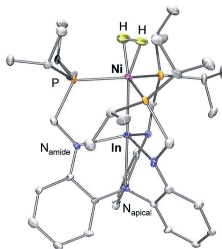
Fig. 1 Neutron structure of 3- \text{H}_2 . Ellipsoids are shown at the 50% probability level, and H atoms (with the exception of \text{H}_2 ) have been omitted for clarity.
