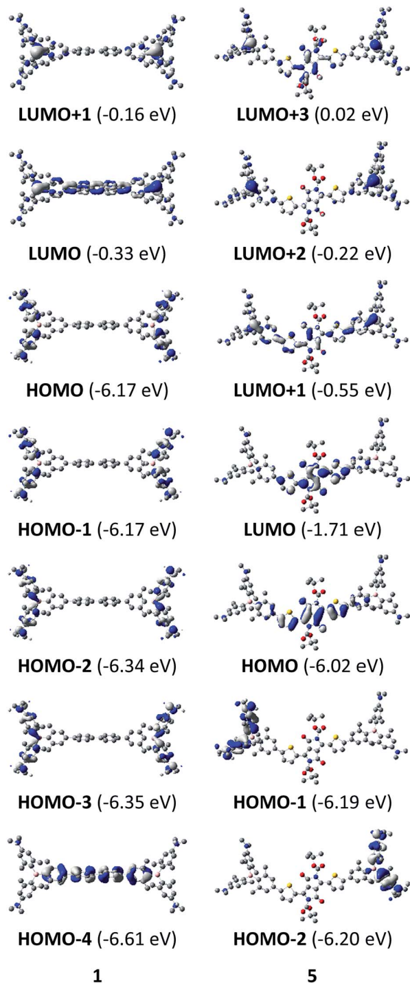
Fig. 2 DFT (CAM-B3LYP/6-31G(d))-calculated relevant orbitals for 1 and 5. Hydrogen atoms are omitted for clarity. Surface isovalue: \pm 0.03 [ \text{e}_0^{-3} ] ^{1/2} . Orbital energy differences are not direct approximations of excitation energies. They are provided here for comparison between the compounds.
