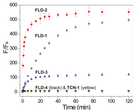
Fig. 4 Fluorescence turn on of FLD-1 (gray), FLD-2 (red), FLD-3 (blue), FLD-4 (black), and TCN-1 (dark yellow) (10 μM) in PBS (pH 7.4, 10 mM) containing Cys (100 μM). \lambda_{\text{ex}} = 490 nm for FLD-1 , 2 , 4 , and TCN-1 , \lambda_{\text{ex}} = 454 nm for FLD-3 , \lambda_{\text{em}} = 500 –650 nm, and slit width = 0.3 nm. The experiments were performed in triplicate. The results are expressed as mean \pm SD ( n = 3 ).
