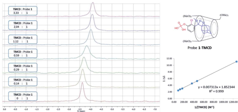
Fig. 5 (Left) ^{31}\text{P} -NMR titration experiment of TMCD and probe 1 . Conditions: 500 \mu\text{L} of \text{D}_2\text{O} , 5 mg of probe 1 and up to 50 mg of TMCD . (Right) Correlation of 1/\Delta\delta as a function of probe 1/[\text{TMCD}] , based on the Benesi-Hildebrand equation.
