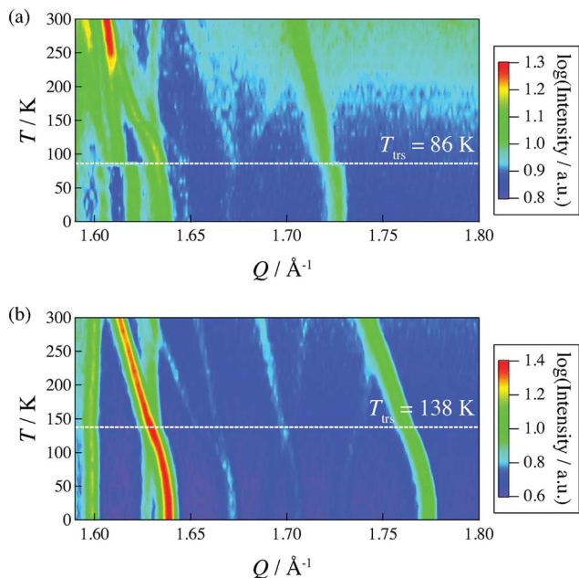
Fig. 19 2-D intensity maps obtained by neutron powder diffraction on IRIS for (a) (NH 4 ) 2 (adp)[Zn 2 (ox) 3 ]·3H 2 O and (b) K 2 (adp)[Zn 2 (ox) 3 ]·3H 2 O. The intensity is given on a logarithmic scale. The white dashed line represents each transition temperature. Reproduced with permission from ref. 77 with permission from Royal Society of Chemistry, Copyright 2014.
