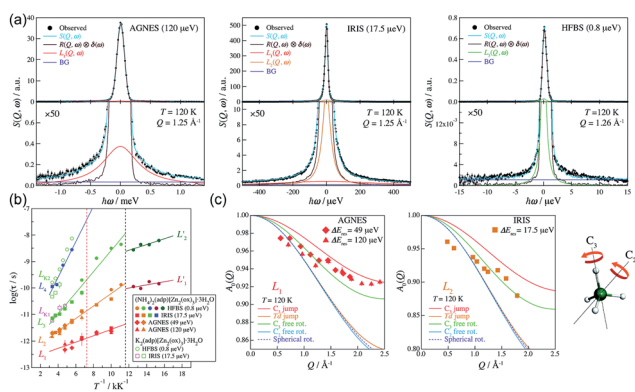
Fig. 20 (a) QENS profiles of (NH 4 ) 2 (adp)[Zn 2 (ox) 3 ]·3H 2 O obtained by using AGNES, IRIS, and HFBS spectrometers. (b) Arrhenius plot for the relaxation times of (NH 4 ) 2 (adp)[Zn 2 (ox) 3 ]·3H 2 O (filled symbols) and K 2 (adp)[Zn 2 (ox) 3 ]·3H 2 O (open symbols) at Q_{\text{av}} = 1.25\text{ Å}^{-1} . (c) EISF of (NH 4 ) 2 (adp)[Zn 2 (ox) 3 ]·3H 2 O for the L_1 mode measured by AGNES (left) and the L_2 mode measured by IRIS (right). Solid curves represent the calculated EISF based on several model functions. Reproduced from ref. 77 with permission from Royal Society of Chemistry, Copyright 2014.
