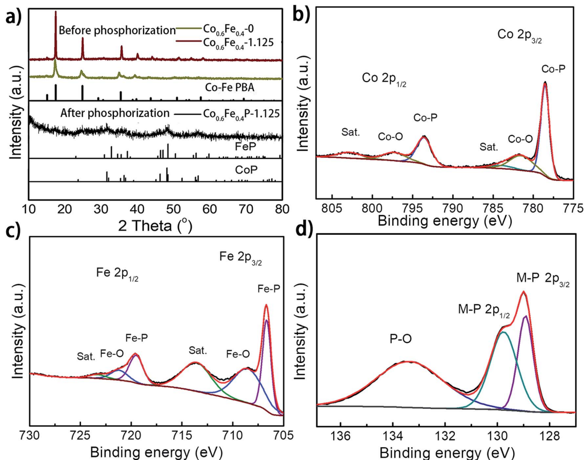
Fig. 2 (a) Powder XRD patterns of the \text{Co}_{0.6}\text{Fe}_{0.4} PBA before and after etching, and the \text{Co}_{0.6}\text{Fe}_{0.4}\text{P} -1.125 after phosphorization; high-resolution XPS (b) Co 2p, (c) Fe 2p, (d) P 2p spectra of the \text{Co}_{0.6}\text{Fe}_{0.4}\text{P} -1.125.
