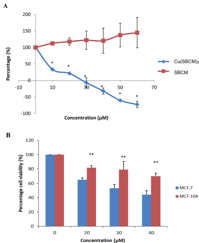
Fig. 2 (A) Effect of SBCM and \text{Cu}(\text{SBCM})_2 on the growth of MCF-7 breast cancer cells as determined by MTT assay. * significantly different from the control SBCM at the same concentration ( p < 0.05 ). (B) Cell viability of MCF-7 and MCF-10A cells after 48 hours exposure with \text{Cu}(\text{SBCM})_2 . ** indicates p < 0.05 when compared between MCF-7 and MCF-10A. Each data point represents the mean of three independent experiments \pm SD.
