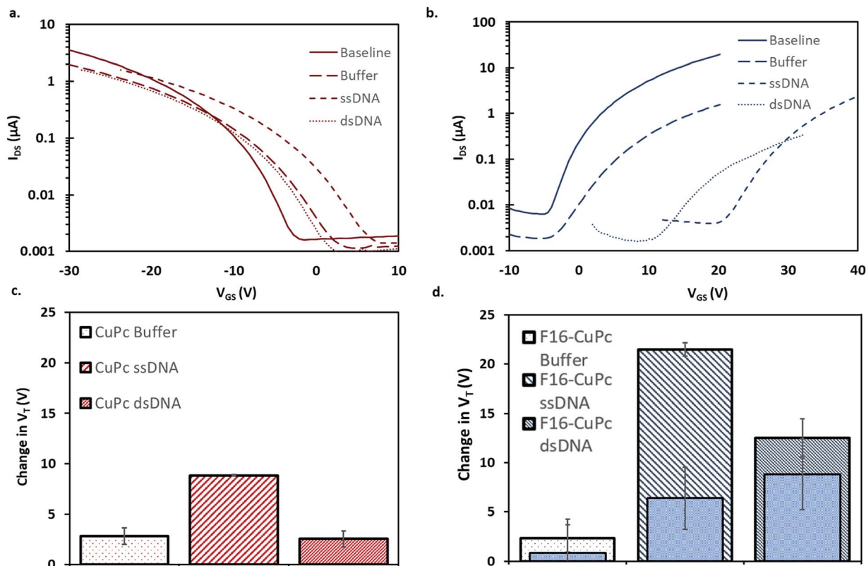
Fig. 6 Transfer curves (a and b) and absolute change in threshold voltage (c and d) of 1 \mu L of 1 \mu M ssDNA, 1 \mu M dsDNA or buffer were added to baseline of CuPc OTFT (a and c) and F 16 -CuPc (b and d). All characterization was performed at 51.1 °C in air except for the superimposed inner bars in (d) (filled blue rectangle) which were characterized at 25.0 °C.
