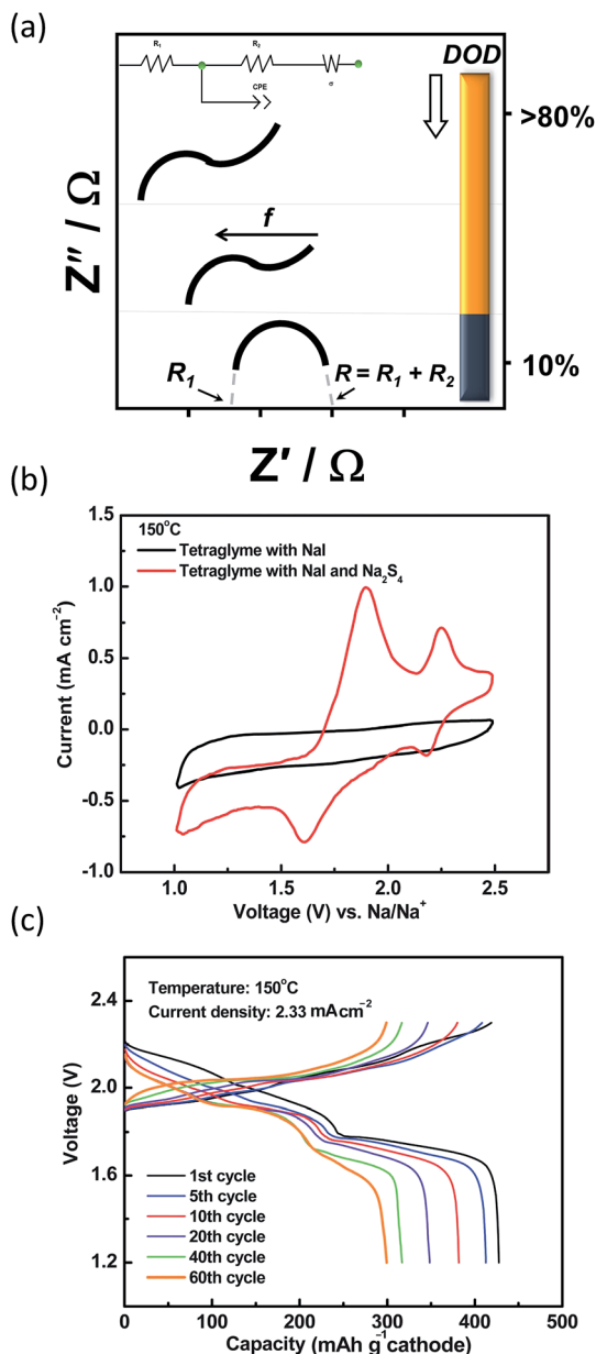
Fig. 14 (a) Nyquist plots of polysulfide melts as a function of depth of discharge (DOD). The diagram is adapted from ref. 212 with permission from Elsevier. (b) Cyclic voltammograms of a planar IT NaS cell containing NaI, TEGDME and \text{Na}_2\text{S}_4 (scan rate: 5 \text{ mV s}^{-1} ). The diagram is adapted/reproduced from ref. 28 with permission from the Royal Society of Chemistry. (c) Cycleability of a IT NaS planar cell (current: 7 \text{ mA} ). The diagram is adapted/reproduced from ref. 28 with permission from the Royal Society of Chemistry.
