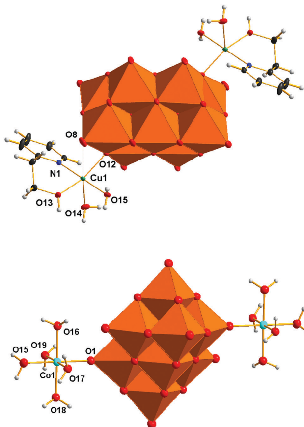
Fig. 1 Molecular structures of the anions [(\text{Cu}(\text{H}_2\text{O})_2(2\text{-hep}))_2\text{V}_{10}\text{O}_{28}]^{2-} ( \text{V}_{10}\text{Cu} ) and [(\text{Co}(\text{H}_2\text{O})_5)_2\text{V}_{10}\text{O}_{28}]^{2-} ( \text{V}_{10}\text{Co} ) as revealed by X-ray crystallography showing atom labelling. Colour code: orange octahedra \{\text{VO}_6\} , green Cu, light blue Co, blue N, red O, black C, gray H. Ellipsoids are displayed at a 30% probability level.
