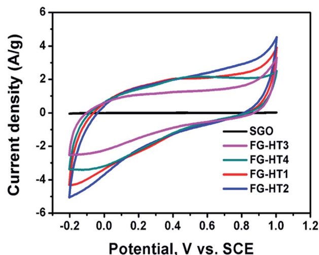
Fig. 11 Cyclic voltammograms of spongy graphene oxide and hydrogenated \text{TiO}_2 with different ratios of functionalized graphene oxide. Reproduced from ref. 117 with permission from the Royal Society of Chemistry.
