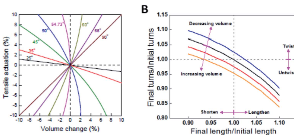
Fig. 15 (A) Calculated tensile strain as a function of volume change for single helices having various initial bias angles. The string length is constant and torsional rotation is prohibited. (B) Values of relative twist ( n/n_0 ) and relative length ( L/L_0 ) that are mutually compatible with the helix model for specified values of an initial helix bias angle of 40°. Blue, black, red, and orange lines are for yarn volume changes of -5\% , 0\% , 5\% , and 10\% , respectively. This figure has been reproduced from ref. 3 with permission from AAAS.
