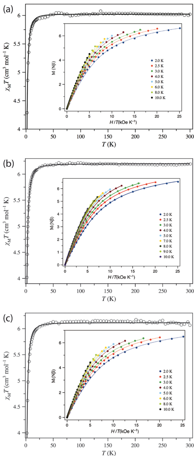
Fig. 5 Plots of \chi_M T vs. T in the range 2–300 K in a 0.025 T ( T < 20 K) and 0.5 T ( T \geq 20 K) applied field and M vs. H/T (inset) for (a) 1 , (b) 2 , and (c) 3 in the 2–10 K temperature range. The solid lines are the best-fit curves, with the fit parameters given in Table 2.
