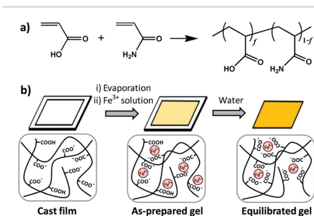
Fig. 7 Diagrams of synthesis of copolymers (a) and physical crosslinked hydrogels (b). Hydrogels were formed by carboxyl-Fe 3+ coordination. The dynamic nature of coordination bonds was rate dependent and the mechanical performance of hydrogels could be tuned by controlling the composition of copolymers, concentration of metallic ions, and pH values of solutions. Reproduced with permission from Macromolecules , 2016, 49 , 9637–9646. Copyright 2016 ACS. 83
