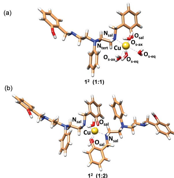
Fig. 3 MOMEc optimized structures for (a) [\text{Cu}^{2+}(\text{2c})(\text{OH}_2)_4] ( 1^2 ; 1 : 1) and (b) [\text{Cu}^{2+}(\text{2c})_2(\text{OH}_2)_2] ( 1^2 ; 1 : 2) complexes. Ligand 2c is in the phenolate form. In the structures, carbon, nitrogen, oxygen and hydrogen atoms are represented in light brown, blue, red and white colors, respectively. Copper ions are represented in gold.
