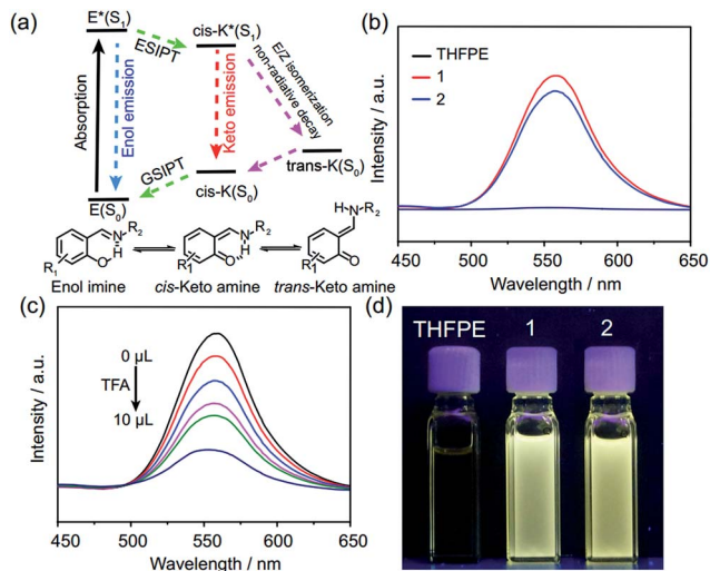
Fig. 4 (a) The ES IPT mechanism of enol-imine compounds through a four-level photo-cycle. (b) Fluorescence spectra of THFPE (30 μM, black), FRSs 1 (10 μM, red) and 2 (10 μM, blue) in chloroform, excited at 360 nm. (c) pH-dependent fluorescence spectra of FRS 1 in chloroform. (d) Fluorescence images of THFPE (1.2 mM, left), 1 (400 μM, middle) and 2 (400 μM, right) under 365 nm UV-irradiation.
