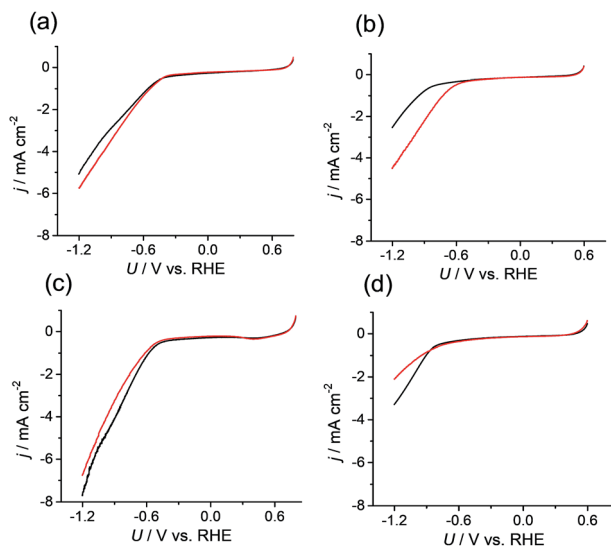
Fig. 2 Current density ( j ) versus potential ( U ) curves obtained from (a) Co-CTF, (b) Ni-CTF, (c) Cu-CTF, and (d) CTF in a phosphate buffer (saturated with Ar, black line) and a \text{KHCO}_3 electrolyte (saturated with \text{CO}_2 , red line).
