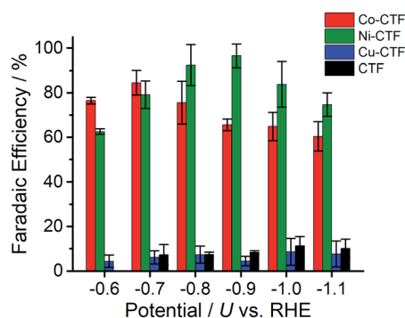
Fig. 3 Effect of potential on the faradaic efficiency values during the \text{CO}_2 RR to generate CO using Co-CTF (red), Ni-CTF (green), Cu-CTF (blue) and CTF (black) in a \text{KHCO}_3 electrolyte (saturated with \text{CO}_2 ) at pH 6.8. The error bar represents the standard deviation from three experimental trial.
