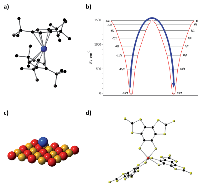
Fig. 5 (a) Molecular structure of [\text{Dy}(\text{Cp}^{\text{ttr}})_2]^+ , where \text{Cp}^{\text{ttr}} = \{\text{C}_5\text{H}_2^t\text{Bu}_3\text{-}1,2,4\} and ^t\text{Bu} = \text{C}(\text{CH}_3)_3 . H atoms are omitted for clarity. Dy: blue and C: black. (b) Energy levels and M_J projections of [\text{Dy}(\text{Cp}^{\text{ttr}})_2]^+ , determined by CASSCF-SO calculations. (c) Ho atom on a MgO monolayer. Mg: yellow and O: red. (d) Molecular structure of [\text{V}(\text{C}_8\text{S}_8)_3]^{2-} . V: red, C: black, and S: yellow.
