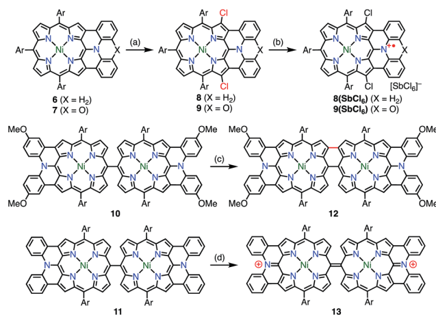
Fig. 5 Diarylamine-fused porphyrins. (a) 2.2 equiv. Palau'chlor, \text{CHCl}_3 , 0^\circ\text{C} to rt, 87% for 6 , 77% for 7 ; (b) 1.1 equiv. magic blue, \text{CH}_2\text{Cl}_2 , rt, 10 min, 79%; (c) 6.0 equiv. magic blue, \text{CH}_2\text{Cl}_2 , rt, 15 min, then \text{H}_2\text{-NNH}_2\cdot\text{H}_2\text{O} , 91%; (d) 2.2 equiv. magic blue, \text{CH}_2\text{Cl}_2 , 10 min, 72%. \text{Ar} = 3,5\text{-di-}t\text{-butylphenyl} .
