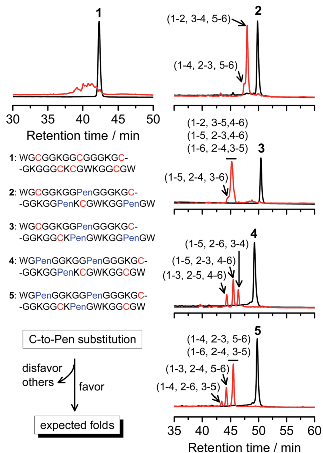
Fig. 2 Amino acid sequences of peptides 1–5 (from N- to C-terminus). Chromatograms showing the oxidation of 1–5 (10 \mu\text{M} ) in 0.2 mM GSSG (100 mM phosphate buffer, pH 7.4) (black line: before the oxidation; red line: 2 h after oxidative folding). C-to-Pen substitutions favor the folding of several expected folds and disfavor the folding of many others (see Fig. 1a). Disulfide pairings were established by tryptic digestion HPLC and mass spectrometry (Fig. S1–S14 † ).
