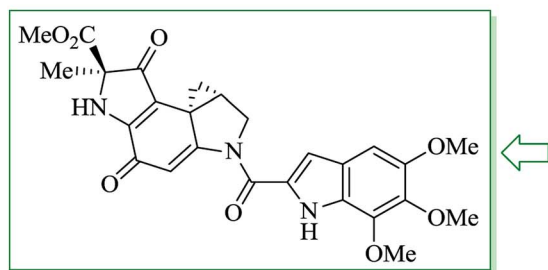
436: Duocannycin A
