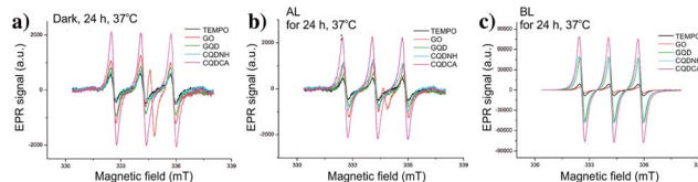
Fig. 5 EPR spectra of GO, GQD, CQDCA and CQDNH with TEMP as a trap, after 24 h at 37 °C in the dark (a), under AL (b) and upon BL exposure (c).
