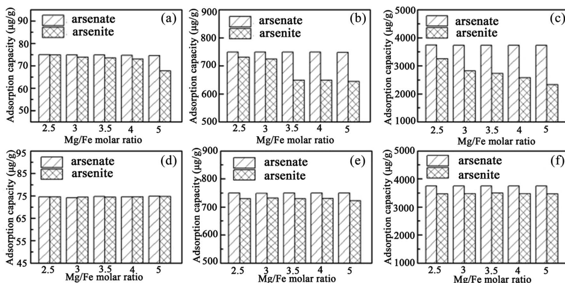
Fig. 8 Comparison of the adsorption capacity between the uncalcined (a–c) and calcined (d–f) iowaitees. (a–c) or (d–f) correspond to the initial arsenic concentrations in solution of 150, 1500, and 7500 \mu\text{g L}^{-1} , respectively (reproduced with permission from ref. 92).
