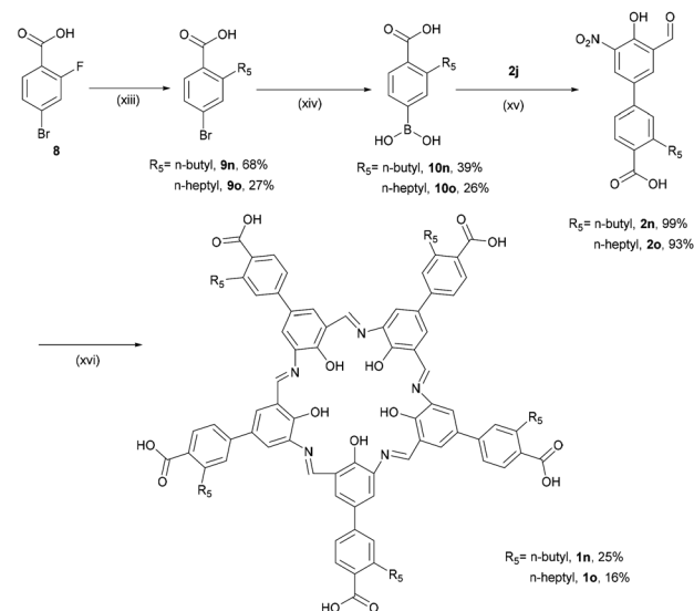
Scheme 3 Syntheses of campestarenes ( 1n and 1o ): (xiii) \text{R}_5\text{MgBr} , \text{THF} , \text{N}_2 , 17 h, then \text{HCl} ; (xiv) n -BuLi, \text{B}(\text{O}-i\text{-Pr})_3 , \text{THF} , -78^\circ\text{C} , 3 h, then \text{HCl} ; (xv) \text{Na}_2\text{CO}_3 , \text{Pd}(\text{PPh}_3)_4 , \text{DMF}/\text{H}_2\text{O} , 105 °C, 6 h; (xvi) \text{Na}_2\text{S}_2\text{O}_4 , \text{EtOH}/\text{H}_2\text{O} , reflux, 2 h.
