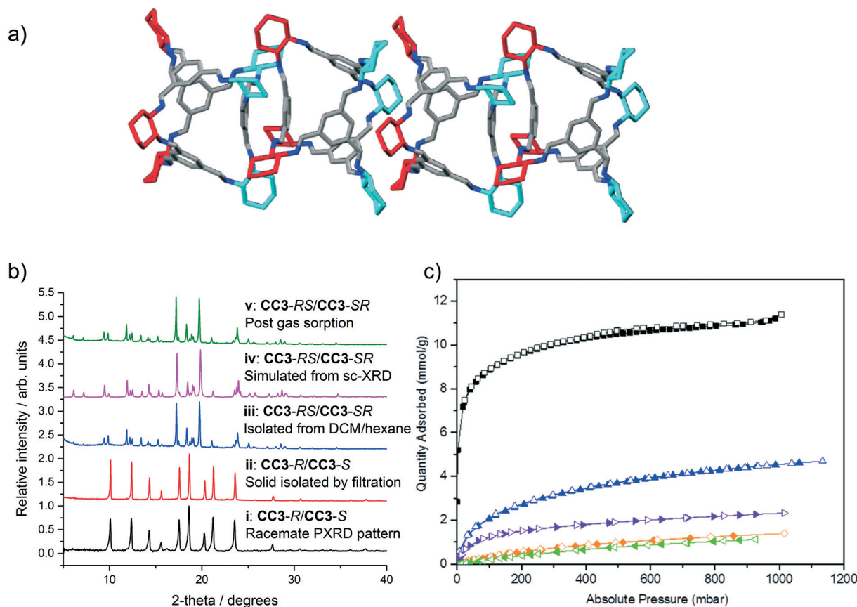
Fig. 4 a) Four cages are shown with both arene-to-arene (leftmost cage pair) and window-to-window packing (central cage pair), taken from the single crystal structure of CC3- RS /CC3- SR (ESI† section 2.8). Hydrogen atoms removed for clarity; colouring as in Fig. 1. b) PXRD patterns of (i) known racemate CC3- R /CC3- S , (ii) CC3- R /CC3- S precipitate isolated via filtration; (iii) CC3- RS /CC3- SR isolated by precipitation with hexane, (iv) simulated PXRD from sc-XRD data for CC3- RS /CC3- SR and (v) CC3- RS /CC3- SR post gas sorption measurements. c) Gas sorption isotherms for CC3- RS /CC3- SR for N 2 (77 K, black), H 2 (77 K, blue), CO 2 (295 K, orange), Xe (273 K, purple), and Kr (273 K, green). Filled and open symbols represent adsorption and desorption isotherms respectively.
