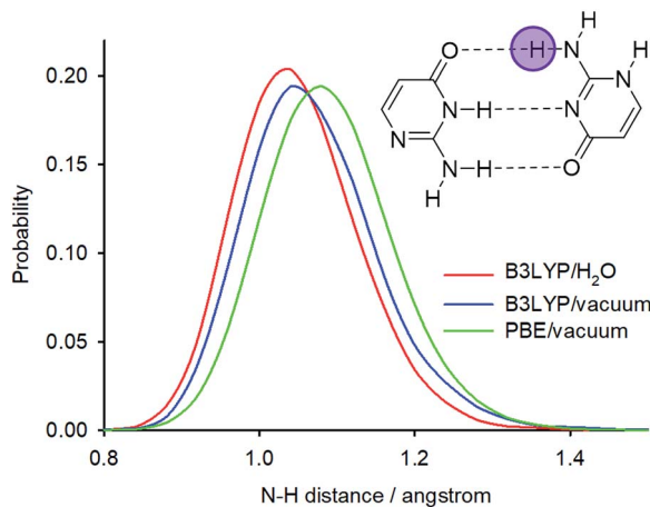
Fig. 8 \text{N2}'\text{-H2}^b distance probability distributions obtained from PIMD simulations at different computational levels.
