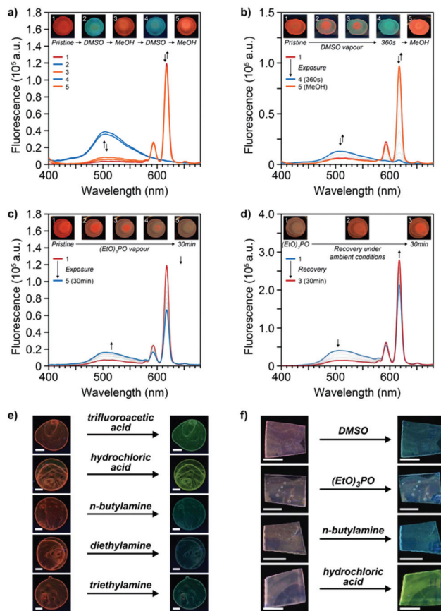
Fig. 4 Fluorescence spectra ( \lambda_{\text{ex}} = 370 nm) and pictures (all taken under illumination with 365 nm UV light) of drop-cast films of the MSP 2:Eu upon exposure to different analytes. (a) 2:Eu in its pristine state (1) and upon consecutive exposure to a drop of DMSO (2,4) and washing with MeOH (3,5). (b) 2:Eu in its pristine state (1) and upon exposure to DMSO vapours (2–4) for up to 360 s, followed by washing with MeOH (5) (spectra normalized at 617 nm). (c) 2:Eu in its pristine state (1) and upon exposure to (\text{EtO})_3\text{PO} vapour for up to 30 min (5). (d) Recovery of the sample shown in (c) under ambient conditions. (e) 2:Eu in its pristine state (left) and upon exposure to trifluoroacetic acid, hydrochloric acid, n -butylamine, diethylamine, as well as triethylamine (right). (f) 2:Eu on an ethylene vinyl alcohol copolymer support in its pristine state (left) and upon exposure to DMSO, (\text{EtO})_3\text{PO} , n -butylamine, and hydrochloric acid (right) (scale bar = 2 mm).
