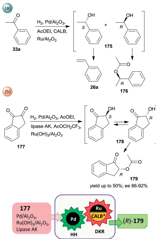
Scheme 50 Cascade reaction of prochiral ketones by HH and KR or DKR using supported Pd, Ru and immobilized lipase catalysts. 220–222
