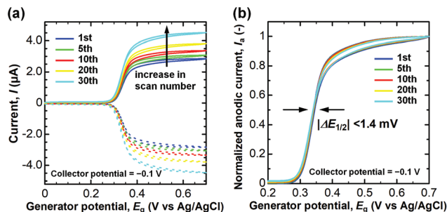
Fig. 8 (a) I_a (solid line) and I_c (dashed line) in 30 times repeated dual-mode CV of DA (100 μM) in PBS (pH 7.4) with the CNTF-IDE ( W_e = 2 \mu\text{m} and W_g = 3 \mu\text{m} ) at v = 10 \text{ mV s}^{-1} . (b) Normalized I_a by that at 0.7 V.
