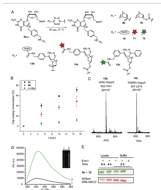
Fig. 2 Reaction of norbornene-modified cap analogs 9b–c in a tetrazine ligation for reaction with biotin-tetrazine or dye-tetrazine conjugates. (A) Scheme for the labeling of norbornene-modified cap analogs 9b–c . (B) Time-course experiments for the reaction of 4-vinylbenzyl or norbornene-modified GpppA with 10 . For each time-point three independent experiments were performed. (C) Mass spectrometric analysis of biotin-GpppA ( 13b ) and TAMRA-GpppA ( 14c ) conjugates. (D) Emission spectra of the OregonGreen-tetrazine conjugate 12 before (black curve) and after reaction with cap analog 9c (green curve), yielding cap analog 15c . A 6-fold fluorescence turn-on was observed (calculated from integration over the area under the curve). Inset: visualization of the turn-on response of 15c by a hand-held UV-lamp ( \lambda_{\text{ex}} : 365 nm). I: tube containing GpppA (300 \mu M) and 12 . II: tube containing 15c (300 \mu M). (E) PAGE analysis of the enzymatic transfer using 1c and subsequent reaction with tetrazine-conjugate 12 in reaction buffer and eukaryotic cell lysate (upper panel). This reaction was compared to enzymatic transfer using 1g , followed by a SPAAC reaction with Sulforhodamine B-DBCO (lower panel). Reaction was performed in reaction buffer and eukaryotic cell lysate.
