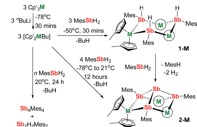
Scheme 1 Synthesis of 1-M and 2-M ( \text{M} = \text{Dy}, \text{Y} ; \text{Mes} = \text{mesityl} ; the circled M represents \text{Cp}'_2\text{M} ).
