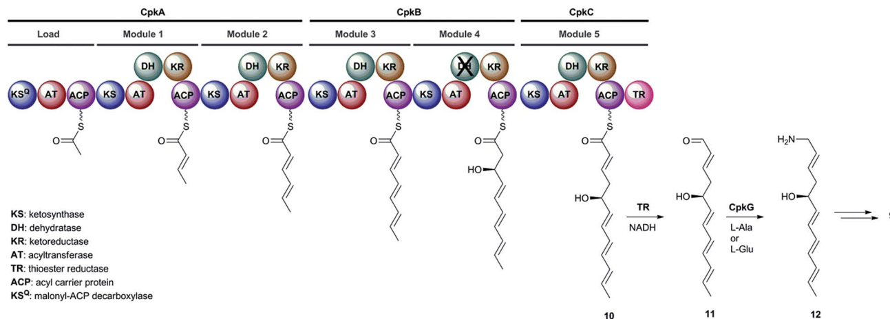
Fig. 2 The proposed roles played by the CpkABC modular PKS and the CpkG ω-transaminase in coelimycin P1 9 biosynthesis.
