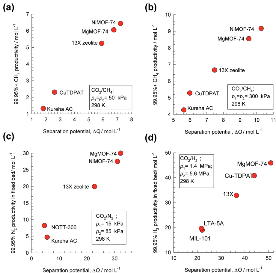
Fig. 6 Plots of the productivity of pure B, of specified purity, versus the separation potential, \Delta Q_{B/A} = Q_A \frac{y_B}{1-y_B} - Q_B , for A/B mixture separations in fixed beds. (a) 50/50 \text{CO}_2/\text{CH}_4 mixture at 100 kPa, (b) 50/50 \text{CO}_2/\text{CH}_4 mixture at 600 kPa, (c) 15/85 \text{CO}_2/\text{N}_2 mixture at 100 kPa, and (d) 20/80 \text{CO}_2/\text{H}_2 mixture at 7 MPa. All calculation details and structural information on the various MOFs are provided in the ESI.†
