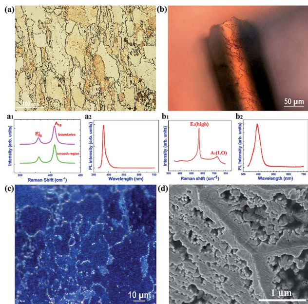
Fig. 5 (a) OM images of the GaN nanowires grown on \text{MoS}_2/\text{Mo} ; ( a_1 ) the Raman and ( a_2 ) PL results of the sample; (b) OM images of the GaN nanowire rolled-up membranes; ( b_1 ) the Raman and ( b_2 ) PL results of the rolled-up membranes; (c) OM images of the GaN nanowire membranes on PET; (d) SEM image of the bottom of nanowires.
