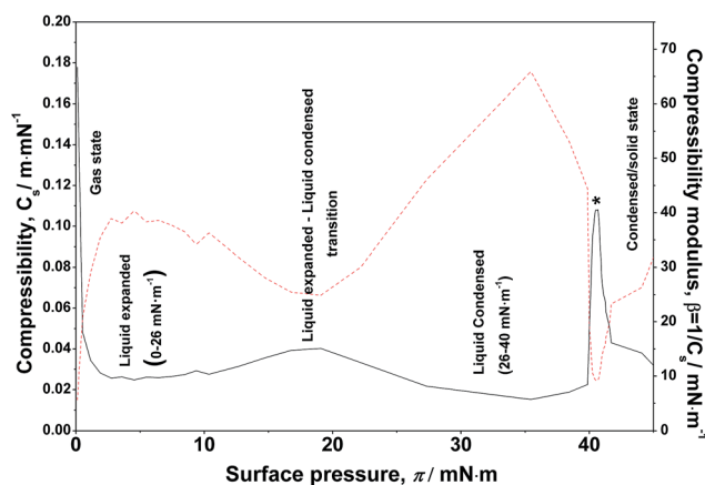
Fig. 3 Lateral compressibility (black line) and compressibility modulus (red-dotted line) –surface pressure diagram for an ODA/DNA mixed monolayer. The DNA concentration was 7.86 \mu\text{M} . All states and transition phases are labeled in the graph.
