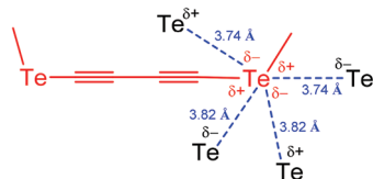
Scheme 2 Multiple chalcogen bonding in 1,4-bis(methyltellanyl)buta-1,3-diyne (one fragment is shown). 41
